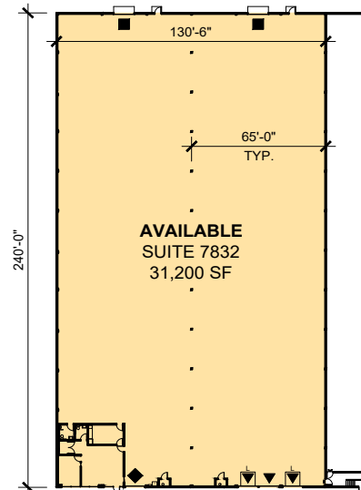
ENLARGED PLAN 1" = 50'-0"
